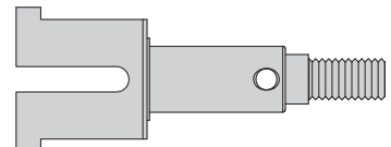
86928 Super Heavy Duty Axle 8x11x44mm Super Heavy Duty Achse 8x11x44mm Essieu Super Renforce 8x11x44mm スーパーHDアクスル8x11x44mm
